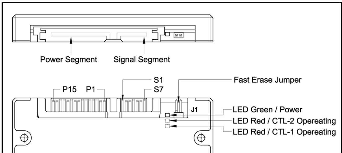
Figure 4: Device – SATA Pins and LEDs Configuration
